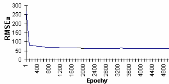
Figure 3: Epochs versus RMSE
