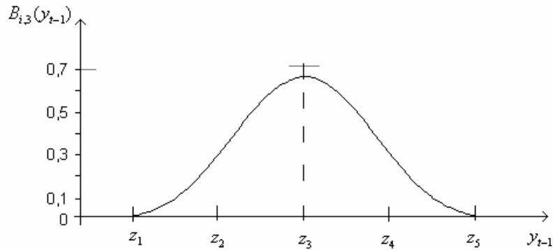
Figure 2: Plot of B-spline values
